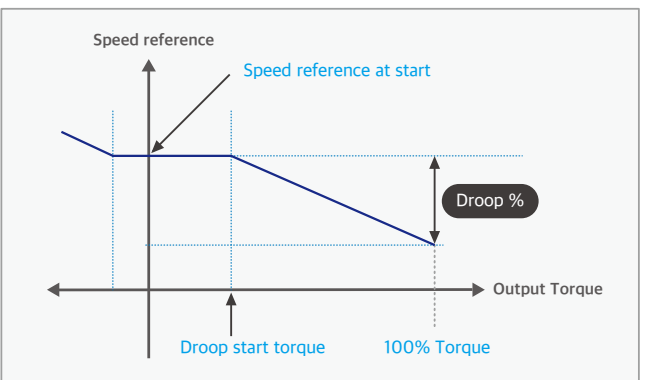
[ Load balancing by droop control ]
